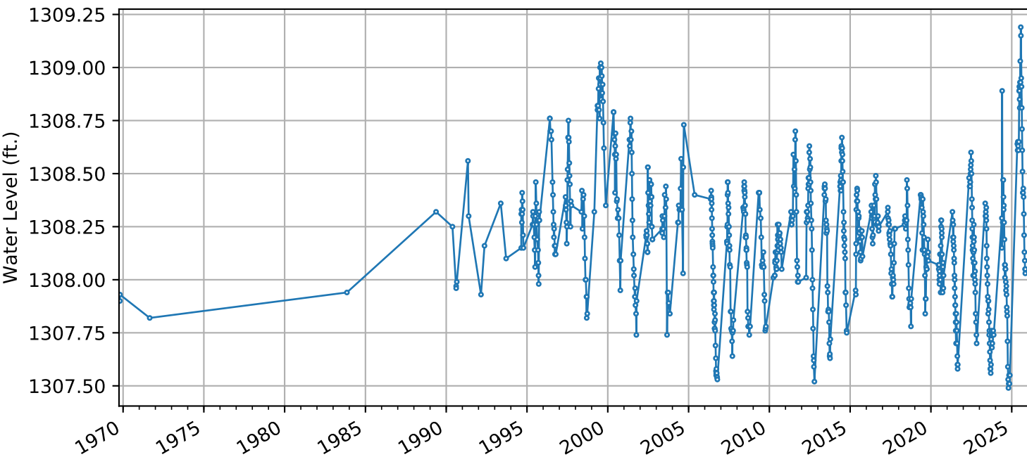
Recorded Water Levels 1969-10-1 to 2025-12-31
